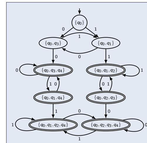
The DFSM accepts the same language but is not necessarily minimal.
