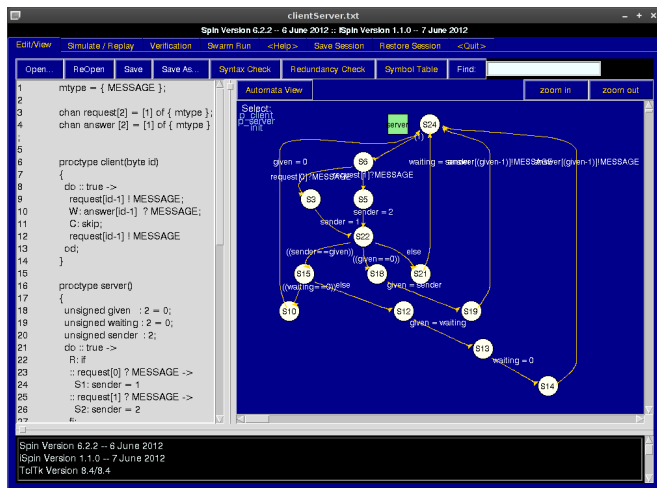
Modeling and verification of concurrent systems.
