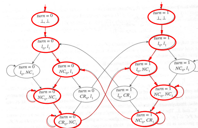
Figure 2.2 Reachable states of Krinke structure for mutual exclusion example.
